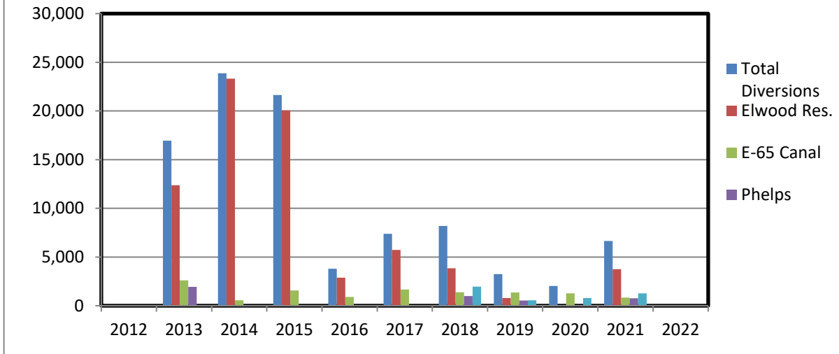
Graph 1: Platte Excess Flow Diversions by CNPPID for TBNRD and NDNR
